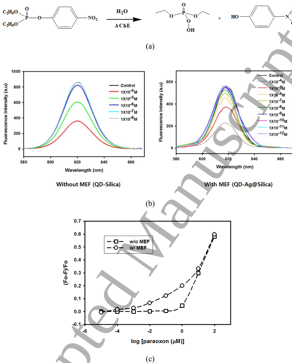
Figure 5. Investigation of the reaction between paraoxon and AChE in solution by monitoring the fluorescence quenching of QDs. (a) Scheme of the reaction between paraoxon and AChE that produce pNP (quencher of QD). (b) Change of fluorescence spectra after the reaction between AChE and different concentration of paraoxon with and without MEF effect. (c) Change of (F_0-F)/F_0 value as a function of paraoxon concentration.
