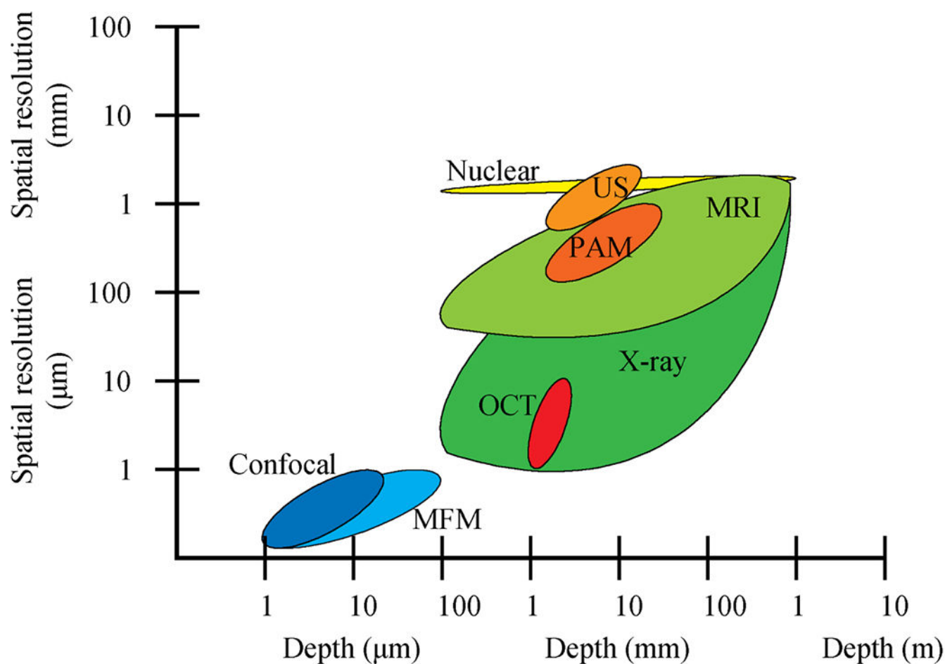
Figure 6. Approximate ranges of spatial resolution and imaging depth achievable by imaging modalities for tissues. US = ultrasound, PAM = photoacoustic microscopy, MRI = magnetic resonance imaging, MFM = multiphoton fluorescence microscopy, OCT = optical coherence tomography. Reprinted from [46], Copyright (2013), with permission from Elsevier.
