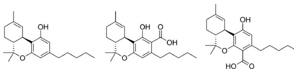
FIG. 1. Chemical structures of THC (left), THCA-A (center), and THCA-B (right). THC, \Delta^9 -tetrahydrocannabinol; THCA-A, \Delta^9 -tetrahydrocannabinolic acid A; THCA-B, 4-COOH-THC.
