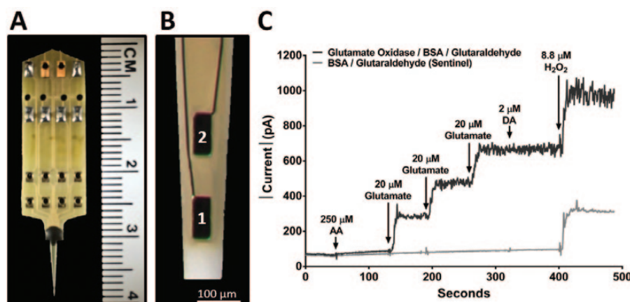
Figure 1. Microelectrode array (MEA) and in vitro calibration. (A) Image of the R2 MEA used for anesthetized recordings with a ruler for scale comparison and (B) magnified tip depicting 2 Pt recording sites, each measuring 50 \times 100 \mu\text{m} with 100\text{-}\mu\text{m} spacing between sites. (C) A typical MEA in vitro calibration measuring the change in current on a glutamate measuring site (black) and a sentinel recording site (gray) with the addition of multiple analytes, as indicated ( \uparrow ). The addition of interferents such as l-ascorbic acid (AA) and dopamine hydrochloride (DA) produced no current change on either site because they are blocked by the mPD exclusion layer. Three glutamate additions showed a stepwise increase of current on the glutamate oxidase/bovine serum albumin (BSA)/glutardialdehyde site, but no response on the BSA/glutardialdehyde sentinel site. The addition of \text{H}_2\text{O}_2 produced a similar increase of current on both recording sites demonstrating equivalent functionality.
