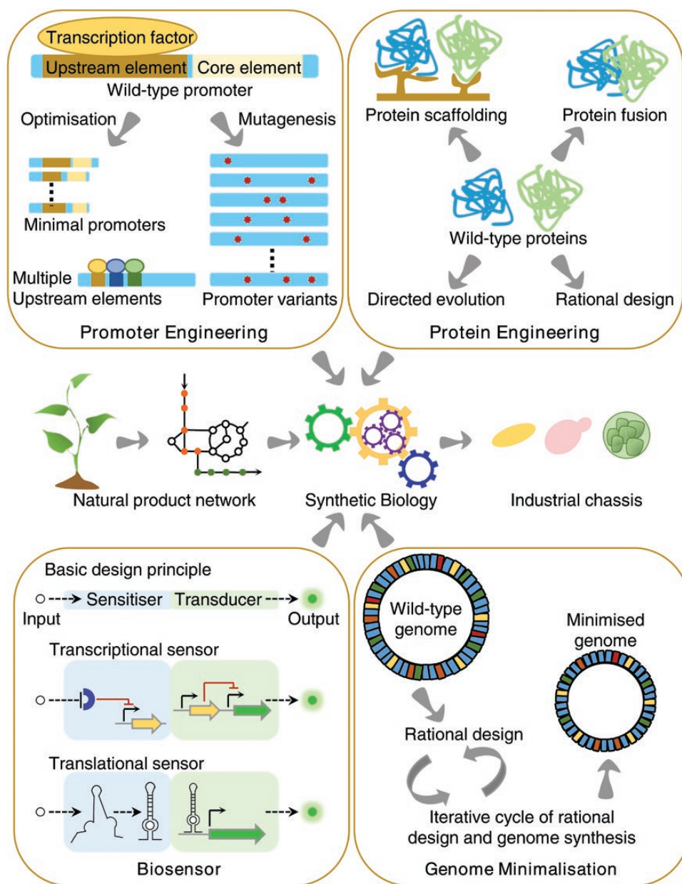
Fig. 2. A schematic overview of the latest synthetic biology tools available for engineering high-value plant natural products in unicellular industrial hosts. For each emerging tool, the basic design principles behind a selection of strategies are depicted.
