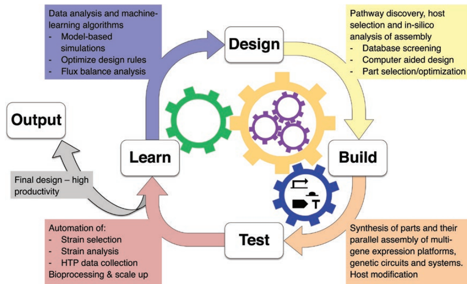
Fig. 1. Schematic representation of the cyclical synthetic biology workflow for metabolic engineering. The workflow is standardized regardless of the DNA components or the host organism, and progresses through iterative cycles of the Design–Build–Test–Learn process to achieve predictable Outputs. In the Design phase, the engineer defines the goal, identifies the pathway(s) and gene(s) of interest, selects host-specific regulatory components (parts) that enable the desired expression of transgene(s), and opts for an assembly approach. The design is implemented in the Build phase and introduced into the host. Evaluating the engineered strains for performance of parts (transcripts and proteins) and production of target molecule(s) generates Test data, which are used during the Learn phase to analyse the components, providing an opportunity to deconstruct complex part combinations and generate knowledge, which can be used for production of tangible and predictable Output(s).
