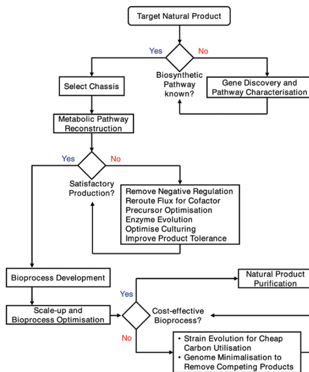
Fig. 4. A concise flow diagram depicting the key steps in engineering unicellular chassis for the production of high-value plant natural products.
