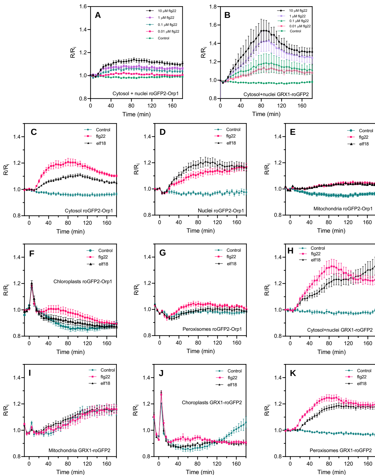
Figure 2 PAMP-induced roGFP2-Orp1 and GRX1-roGFP2 redox dynamics in different subcellular compartments. Dose–response kinetics of cytosolic/nuclear roGFP2-Orp1 (A) and GRX1-roGFP2 (B) oxidation in leaves in response to the PAMP flg22. Leaf discs were exposed at t = 0 min to control solution or different concentrations of flg22. The 400/485 nm fluorescence ratio ( R ) was measured over time by multiwell fluorimetry and expressed relative to the mean initial ratio ( R_i ) before treatment. Data are means \pm SE from a representative experiment ( n = 6 ). The experiments have been repeated at least twice with similar results. Kinetics of roGFP2-Orp1 oxidation in the cytosol (C), nuclei (D), mitochondria (E), chloroplasts (continued)
