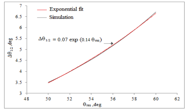
Fig. 5. Illustration of \Delta\theta_{1/2} for various resonance incidence angles with rectangular grating configurations in the GG-SPRB.
