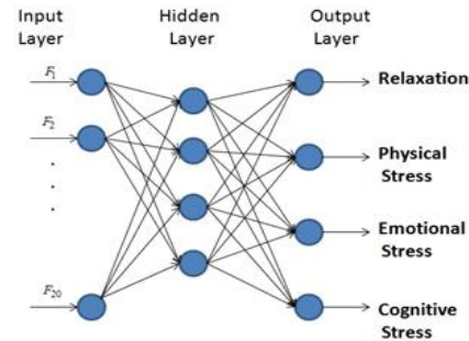
Fig. 2: Neural Network
