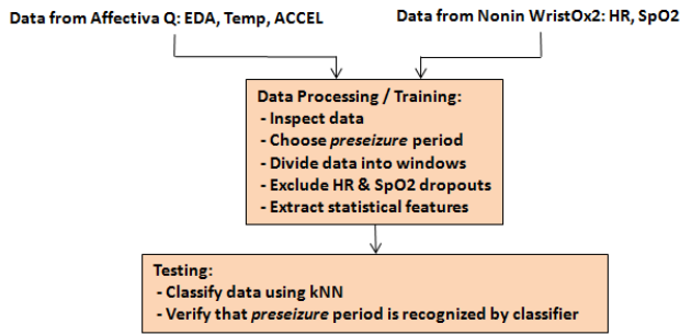
Fig. 3: Procedure for Analyzing Seizure Data
