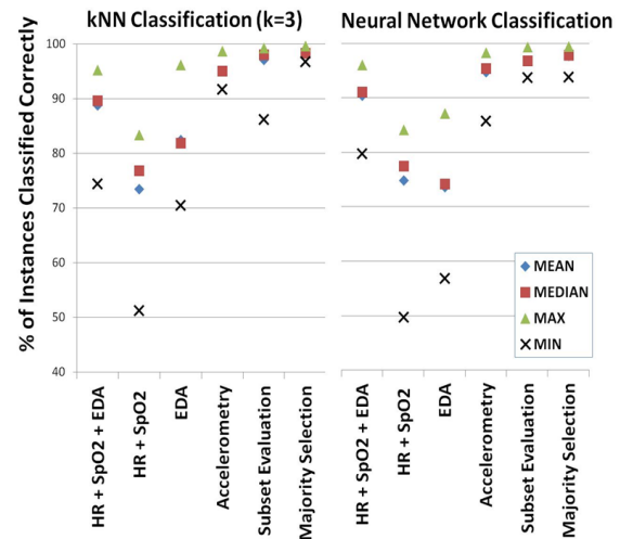
Fig. 5: 20 Subject Classification Using (a) kNN, (b) Neural Network
