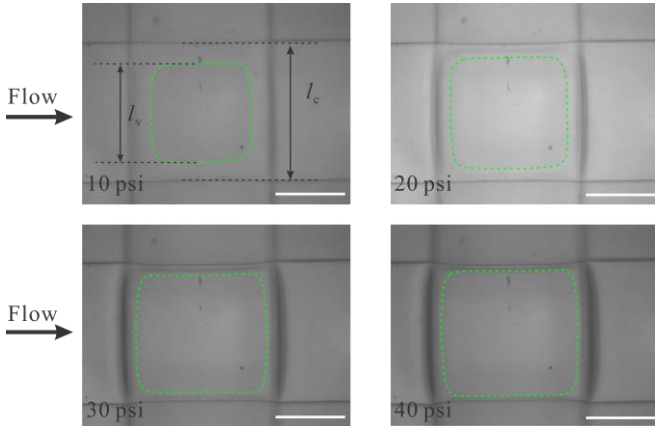
Figure 3. Images comparing valves operation at different pressures. The images show the top views of valves. The white scale bars are 300 \mu\text{m} . The green dash lines denote the part of valves that are closed. l_c is the width of flow channel and l_v is the width of the closed part of valve.
