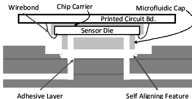
Fig. 4. Schematic drawing of the cross section of the interface between the Lab Card (bottom) and the PCB carrying a GMR sensor die in a microfluidic package. As in other Figs., the closest ports are separated by 2.0 mm. The port diameters are designed to be 200 microns in diameter, which places an upper limit of about 100 microns on allowable misalignment between the card and microfluidic chip while still having adequate flow path.
