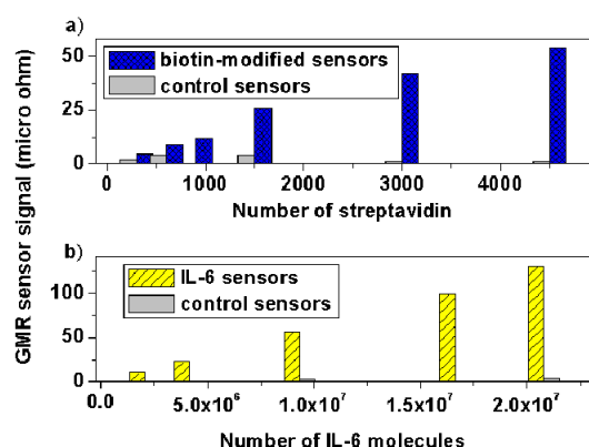
Fig. 6. a) Resistance change for different amounts of streptavidin molecules on the GMR sensor. Blue: GMR sensors with surface modified by biotin. Gray: GMR sensors with no biotin modification. b) Resistance change detected by sensors for different amounts of IL-6 molecules modified on the sensors using a sandwich structure. The same amount of capture antibody and detection antibody-modified magnetic nanoparticles was applied to each sensor with varied numbers of IL-6 molecules. Yellow: IL-6 modified GMR sensors. Gray: GMR sensors with no IL-6 modification.
