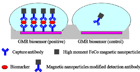
Fig. 2. A novel biomarker detection scheme using GMR biosensor and high moment FeCo magnetic nanoparticle
