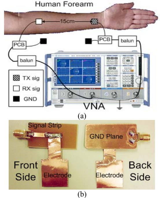
Fig. 3. (a) the measurement setup, port 2 of VNA is TX and port 1 is RX, baluns are used to separate the GND of TX and RX; and (b) the picture of TX and RX PCB boards, the copper-foil-made electrode is soldered to the micro-strip which has characteristic impedance of 50Ω.
