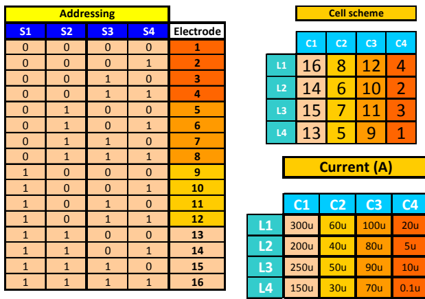
Fig. 2. Addressing table, the corresponding addressed cells in the array and their current.
