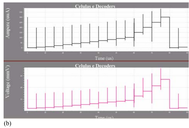
Fig. 4. (a) Schematic of the transimpedance amplifier and (b) its operation showing the output voltage as a function of the input current.
