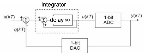
Fig. 6 Block diagram of the one bit first order Sigma-Delta modulator.
