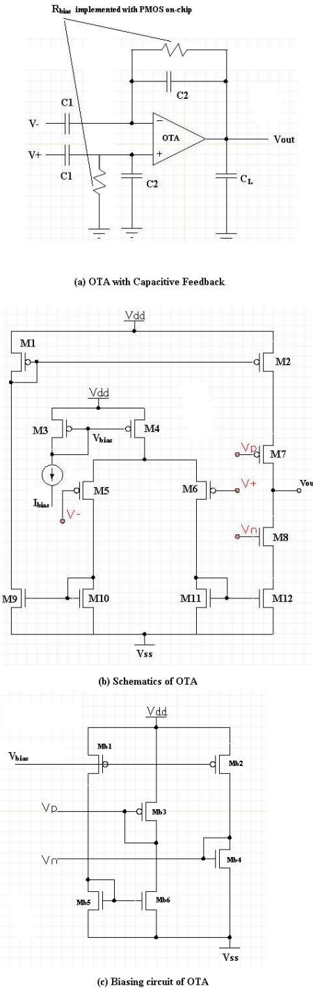
Fig. 3. Schematics of the OTA based high-gain amplifier.
