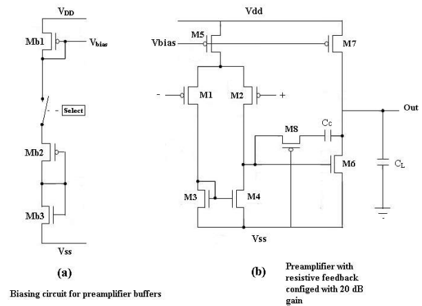
Fig. 2. Schematics of the preamplifiers.
