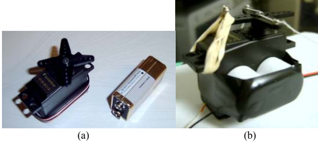
Fig. 2. Original (a) and modified wearable servo motor (b).
