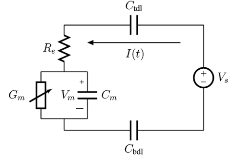
Fig. 2. Schematic of the lumped circuit model for the tethered membrane platform, circuit parameters are defined in Section II-B.
