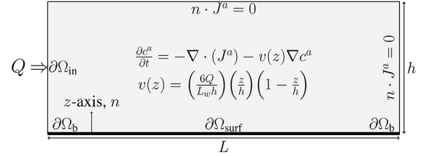
Fig. 4. Schematic of the ICS biosensor model (3a), (4), (5), and (6) with boundary conditions (7). The analyte enters the ICS at \partial\Omega_{\text{in}} with a flow rate of Q . \partial\Omega_{\text{surf}} is the surface of the tethered membrane, and \partial\Omega_b denotes the boundary of the membrane. n denotes the inward normal vector from the surface. Other parameters are defined in Table I.
