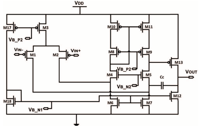
Fig. 5. Folded cascode-Miller OTA circuit.
