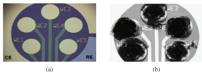
Fig. 10. Chip with multiple gold WE, a common platinum RE and gold CE. (a) Unspotted. (b) Spotted with CNT-based films: Nafion-MWCNT on WE1-W3-W5 and MDB-CHIT-MWCNT-GDH on WE2-WE4.
