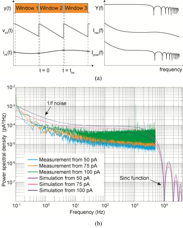
Fig. 4. Characterization of noise using simulation and chip measurement. (a) The current integration creates windows for each integration period and reports the current level at the end of each integration cycle. The window in time-domain generates a sinc() function in the frequency domain which can be used to estimate the noise performance in the non-stationary circuit. (b) Noise analysis from the simulation is compared with the chip measurements for various input current levels, 50 pA, 75 pA and 100 pA.
