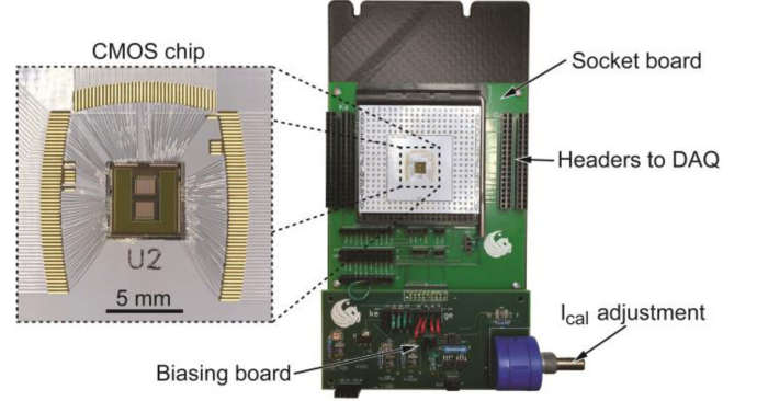
Fig. 5. Overview of the measurement system. The CMOS chip is bonded to a PCB which is inserted into a socket on the socket board. The socket board allows for connections to the National Instruments DAQ unit and to the biasing board. The biasing board converts battery or power supply voltage into V_{DD} , V_{\text{reset}} , V_{\text{pos}} , and I_{\text{cal}} . I_{\text{cal}} is easily adjustable via the 10-turn potentiometer.
