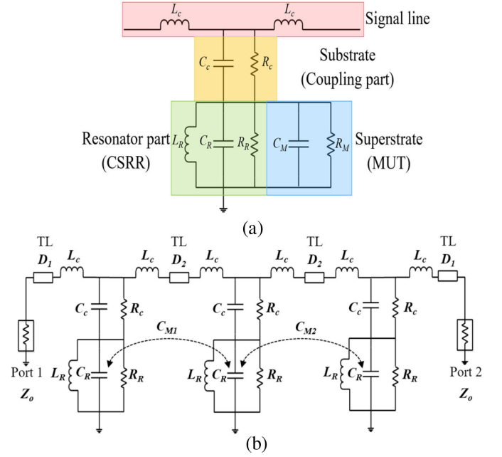
Fig. 3. Equivalent electrical model of (a) single CSRR cell under loading condition, (b) unloaded triple-pole CSRR.
