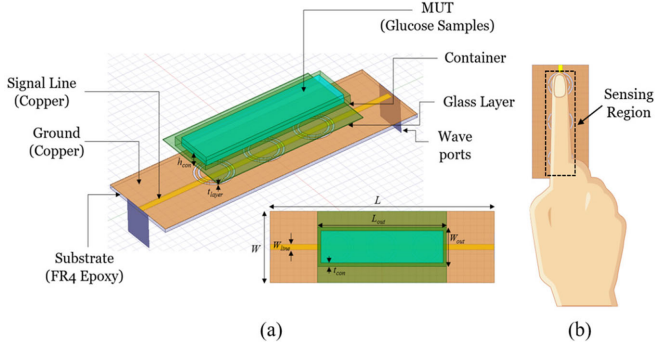
Fig. 10. (a) Geometrical schematic model of the TP-CSRR integrated with the vein-resembling channel (top view of the integrated sensor is enclosed), (b) sensor application for continuous glucose monitoring from the finger.
