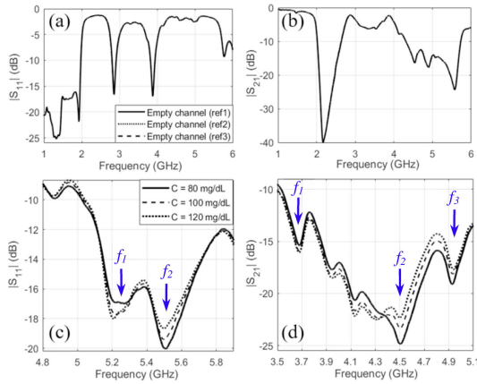
Fig. 16. Measured (a) reflection and (b) transmission coefficients over a broad band 1–6 GHz for the empty channel-loaded sensor. Measured (c) reflection and (d) transmission coefficients for the tested glucose samples on the higher frequency regions.
