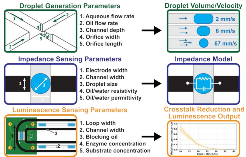
Fig. 4. Droplet microfluidics device parameters for droplet generation, impedance sensing, and luminescence sensing.
