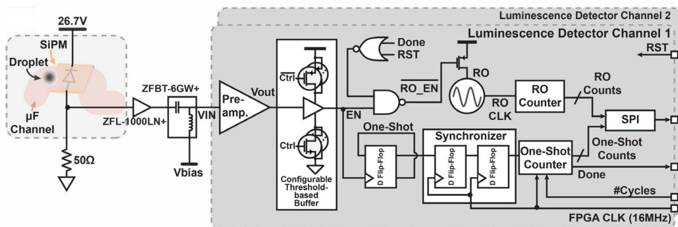
Fig. 11. Luminescence detector architecture.
