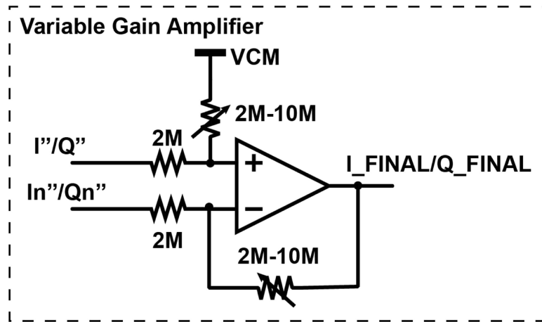
Fig. 10. Variable-gain amplifier implementation.
