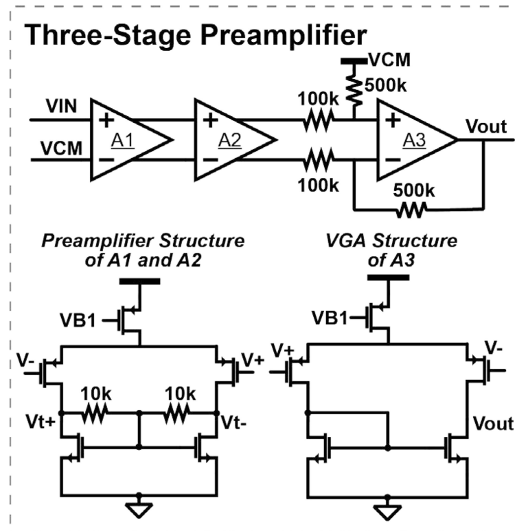
Fig. 14. Three-stage pre-amplifier implementation.
