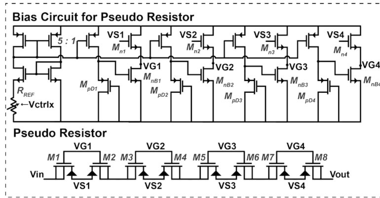
Fig. 9. Temperature- and process-compensated pseudo-resistor implementation.
