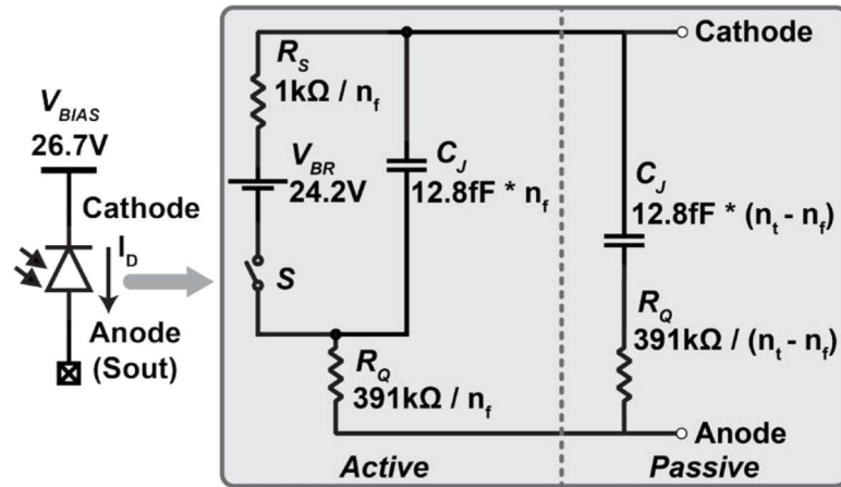
Fig. 13. Equivalent electrical circuit model of the SiPM.
