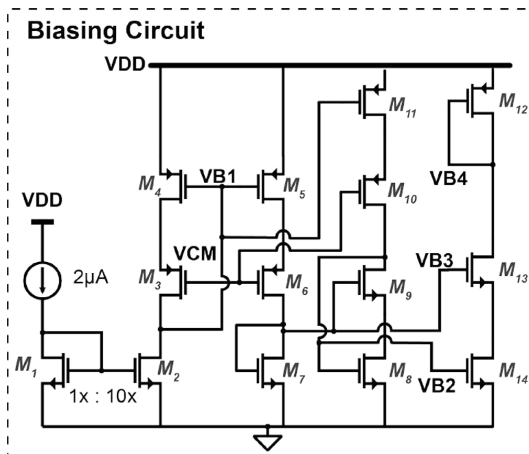
Fig. 8. Bias circuit of the transimpedance amplifier.
