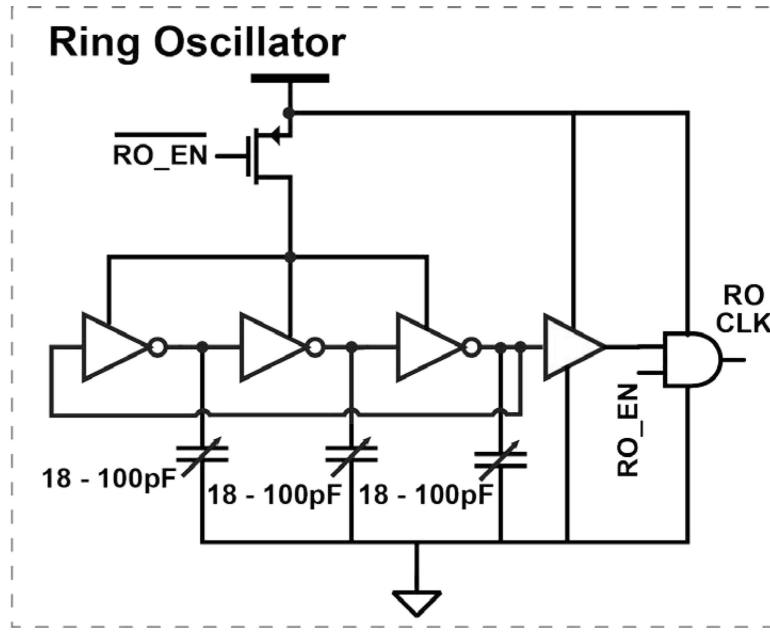
Fig. 15. Ring oscillator implementation.
