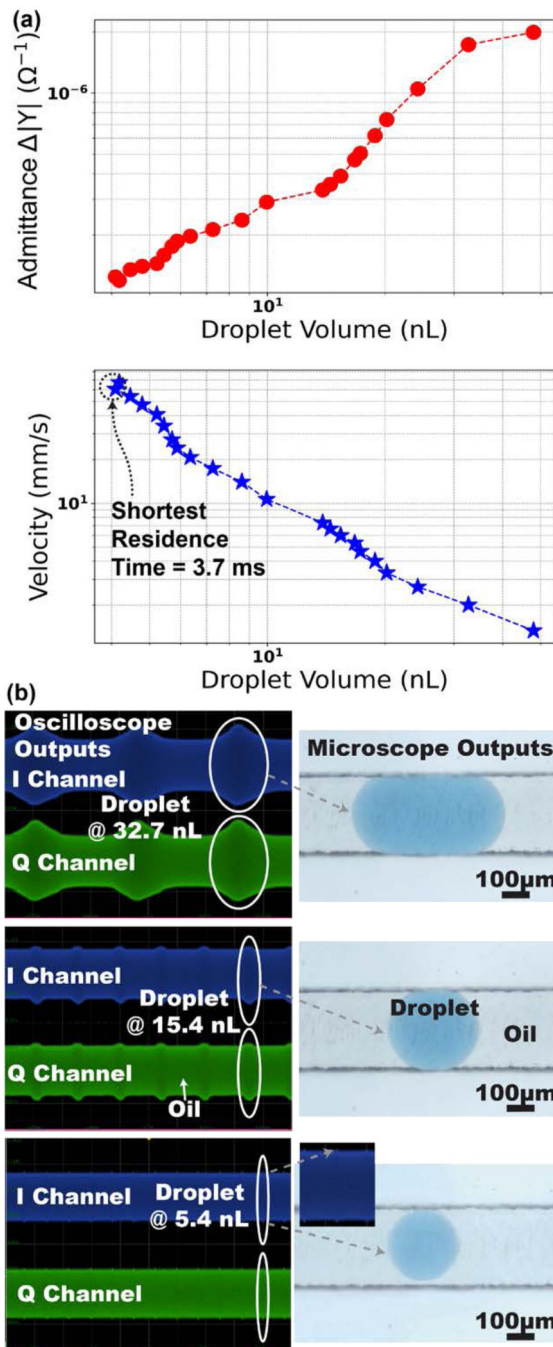
Fig. 20. Real-time droplet detection using the impedance spectroscopy chip.
