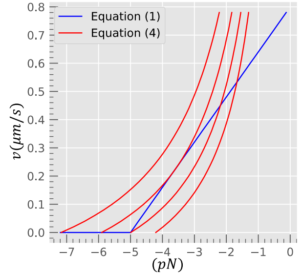
Fig. 5. Plots for microtubule-based molecular shuttles of the gliding speed, v , as a function of impedance given by (4) with various active motor ratios, r (red curves), overlaid with the f-v relation of (1) (blue line). The active motor ratio is 0.328, 0.372, 0.412, and 0.454 from left to right. The critical active motor ratio in this case is 0.372.
