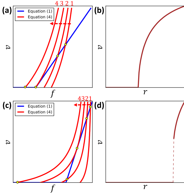
Fig. 3. (a, c) Schematic plots of the gliding speeds as functions of impedance given by (4) with various active motor ratios, overlaid with the f-v relation of (1). (b, d) Gliding speeds, v , as function of active motor ratio, r . (a) and (b): continuous, (c) and (d): discontinuous. The arrows in (a) and (c) point to the direction of increasing \rho_d/\rho_a .
