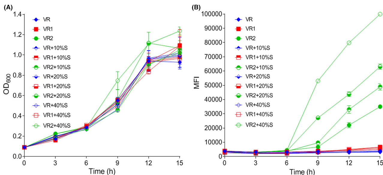
FIGURE 1 The growth curves of VFM biosensors (A) and their responses to the VFM signal (B). VR, VR1 and VR2 indicate \Delta zmsA(pPROBE-NT) , \Delta zmsA\Delta vfmE(pVfmEpro-gfp) and \Delta zmsA(pVfmEpro-gfp) , respectively. The MFI values of VR, VR1 and VR2 biosensors after adding with different concentrations of signal crude extracts (%) were measured by multifunctional microplate reader every 3h.
