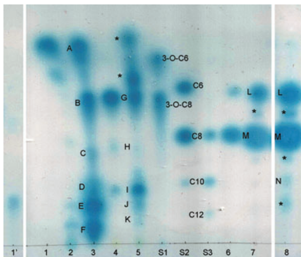
Fig. 5. Analytical TLC assay. S1, S2 and S3, synthesized standards (Sigma, Aldrich): S1, 3-O-C6 HSL (2 pmol) and 3-O-C8 HSL (0.1 pmol); S2, C6 HSL (4000 pmol), C8 HSL (100 pmol), C10 HSL (500 pmol); S3, C8 HSL (20 pmol), C10 HSL (1000 pmol) and C12 HSL (9000 pmol). 1', 1–8, condensed extractions of different strain cultures: 1', HC103(pJZ381)(pQS6-1) (10 ml); 1, HC103(pJZ381)(pQS6-1) (5 ml); 2, HC103(pJZ381)(pRK6-1LuxI) (5 ml); 3, BL21(DE3)(pET6-1LuxI) (2 ml); 4, HC103(pJZ381)(pQS10-1) (5 ml); 5, BL21(DE3)(pET10-1LuxI) (5 ml); 6, HC103(pJZ381)(pQS10-2) (5 ml); 7, BL21(DE3)(pET10-2LuxI) (3 ml); 8, BL21(DE3)(pET10-2LuxI) (5 ml). The numbers in parentheses are the corresponding volume of culture supernatant extracted. The spots labelled from A to N were purified from preparative TLC plates and further analysed using ESI MS and MS/MS. The spots labelled with an asterisk '*' were unknown compounds and were not analysed using ESI MS and MS/MS.
