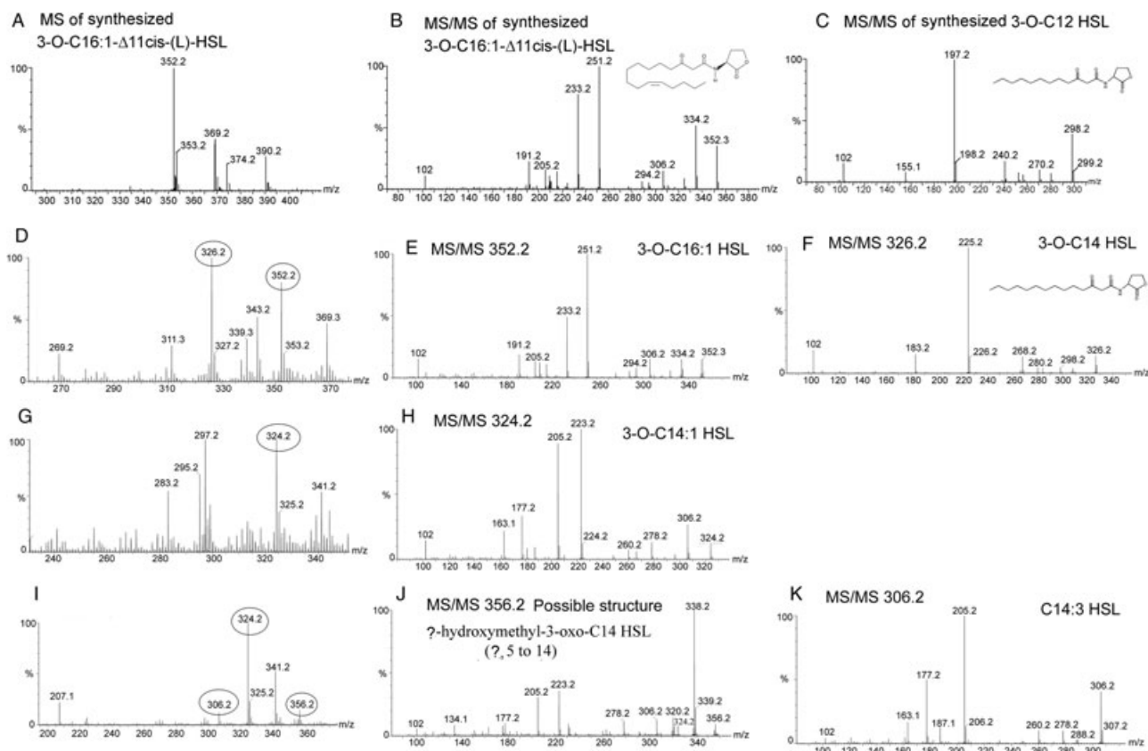
Fig. 6. ESI MS and MS/MS results of the active compounds produced by LuxI QSS-1 (at spot D, E and F on Fig. 5).
