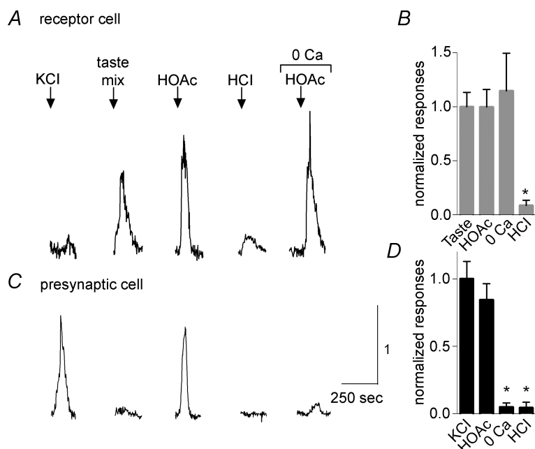
Figure 1. Acetic acid taste stimulation evokes \text{Ca}^{2+} responses in receptor (Type II) cells and presynaptic (Type III) cells
