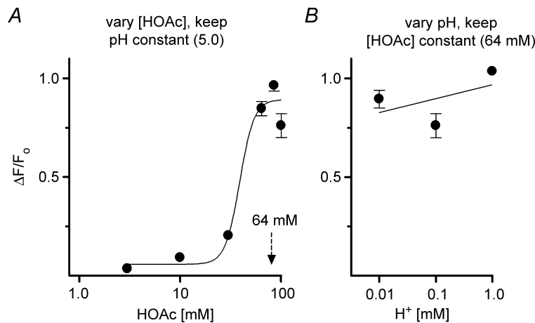
Figure 5. The amplitude of acid-evoked \text{Ca}^{2+} responses varies with [HOAc] but not with [\text{H}^+] (i.e. pH)
