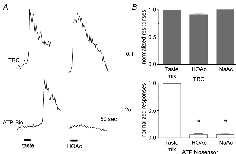
Figure 7. Acid taste stimulation does not evoke ATP secretion from receptor (Type II) cells
