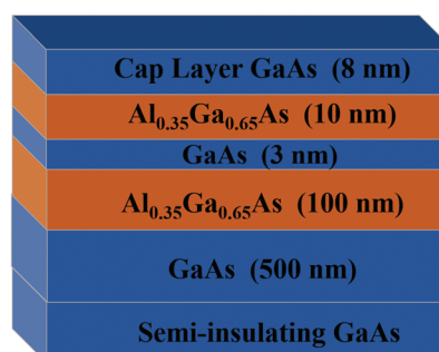
FIG. 1. Schematics of GaAs/ \text{Al}_{0.35}\text{Ga}_{0.65}\text{As} quantum-heterostructures studied in this work.
