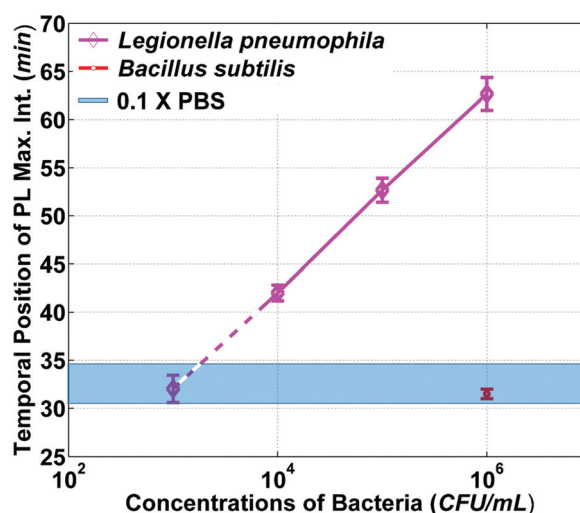
FIG. 8. PL intensity maximum vs time for numerous repeated detection runs.
