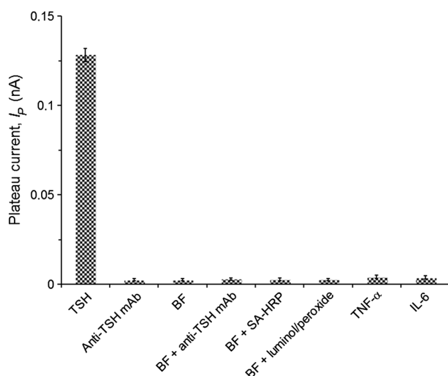
Fig. 6 Specific detection of TSH by the polycarbazole photodetector integrated microfluidic device. The specificity tests were performed with respect to various reagent blanks, analyzing the interference from monoclonal antibody (mAb), blocking buffer (BF), streptavidin-horseradish peroxidase conjugate (SA-HRP) and luminol/peroxide working solution. The negative controls were the cytokines human tumor necrosis factor-alpha (TNF- \alpha ) and human interleukin-6 (IL-6) while the positive control was 2 ng/ml TSH. The error bars represent standard deviation for triplicate tests.
