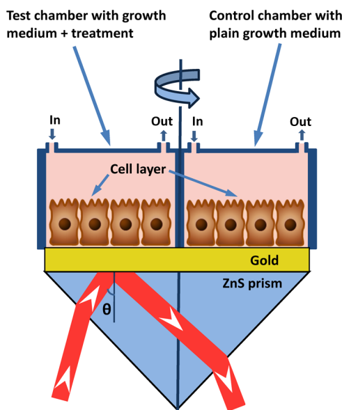
Fig. 1 A double-chamber flow cell for Fourier Transform Infrared-Surface Plasmon Resonance (FTIR-SPR) measurements of living cells. The cell sample is grown homogeneously on the prism surface and is divided into two halves with a separating barrier only at the measuring stage. One chamber undergoes treatment with some stimulus while another chamber serves as control. The infrared beam is reflected from one half of the prism base and its intensity is measured. This yields information on the refractive index of the cell layer in the corresponding chamber. After each measurement, the prism is rotated 180 deg around the vertical axis, and reflectivity from the other chambers is measured (control). Then the prism is rotated -180 deg backward to the initial position and the measurement is repeated. The minimal temporal resolution of our measurements is \sim 1.5 min (40 s for one-channel measurement and 20 s for switching between the channels).
