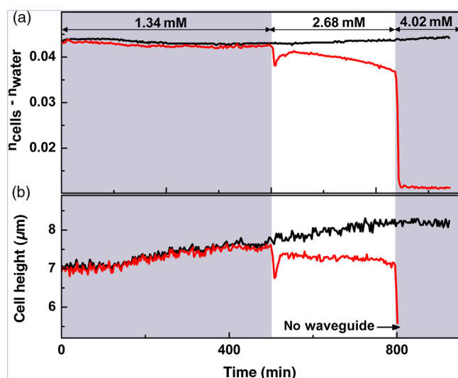
Fig. 5 Dynamics of IEC-18 cells refractive index n_{\text{cell}} (a) and average cell height (b) under prolonged exposure to different concentrations of EDTA. Red line corresponds to the chamber with low \text{Ca}^{2+} (treatment) and black line corresponds to the chamber with normal concentration of \text{Ca}^{2+} (control). Duration of the first stage (1.34 mM of EDTA) is 500 min. Duration of the second stage (2.68 mM of EDTA) is 300 min. Duration of the third stage (4.02 mM of EDTA) is 100 min. The temporal resolution of these measurements is 3 min.
