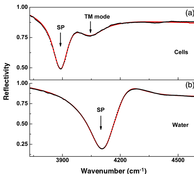
Fig. 2 Measured infrared reflectivity spectra (black dots) and fitting using Fresnel formulae for reflectivity from a multilayer (red solid line): (a) ZnS prism/gold/cells, (b) ZnS prism/gold/water. The nominal gold film thickness is 18 nm and the angle of incidence is 35 deg. The surface plasmon (SP) and TM-waveguide mode resonances are shown by arrows.
