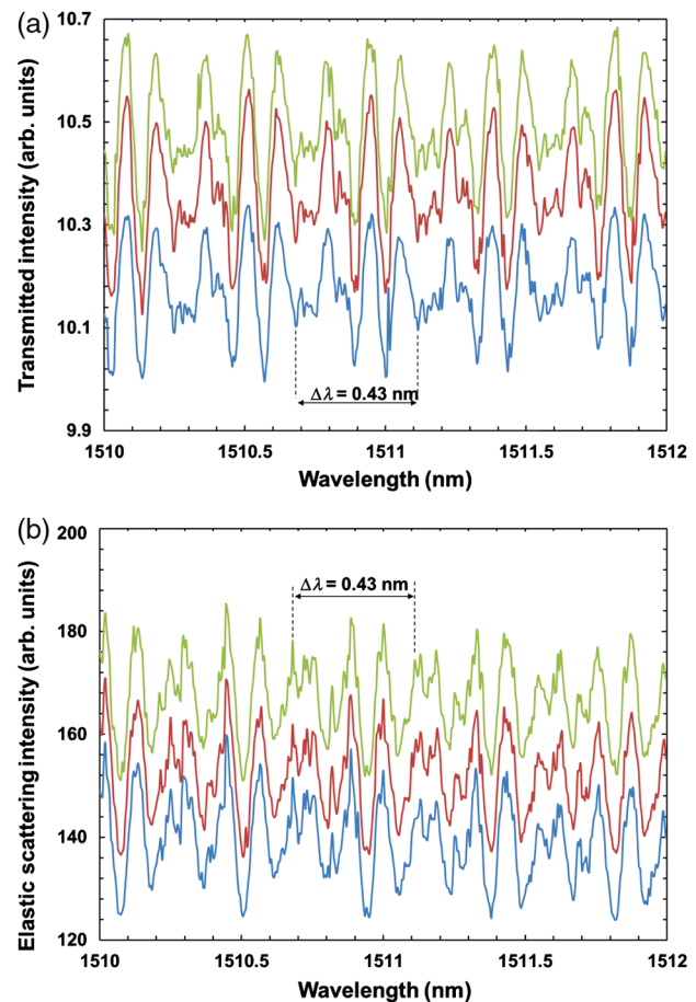
Fig. 3 Transmitted intensity (a) and elastic scattering intensity (b) spectra from nonmodified sapphire sphere repeated three times in order to demonstrate the reproducibility of the concept. Spectra were offset in order to distinguish them in one graph.
