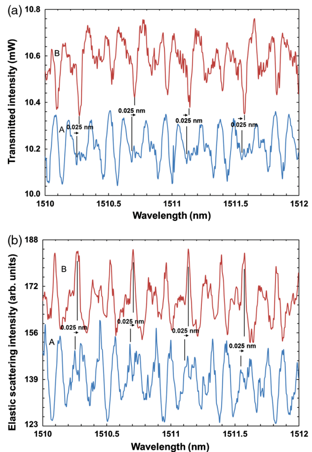
Fig. 7 Transmitted intensity (a) and elastic scattering intensity (b) spectra from sapphire sphere after dsDNA is denatured and the corresponding shift. (A) Nonmodified sphere. (B) DNA modified sphere after denaturation of dsDNA to ssDNA.
