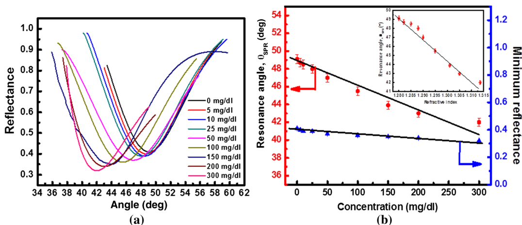
Fig. 6 (a) SPR reflectance curves for prism/Au/ZnO/Urs/buffer system for increasing concentration of urea from 0 to 300 mg/dl and (b) variation of resonance angle ( \theta_{\text{SPR}} ) and minimum reflectance with the concentration of Urs.
