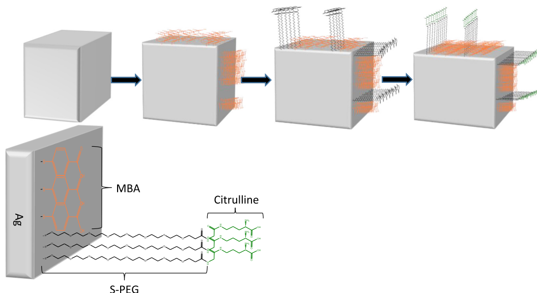
Fig. 1 3-D diagram of process to modify the surface of Ag nanocubes with MBA and citrulline.
