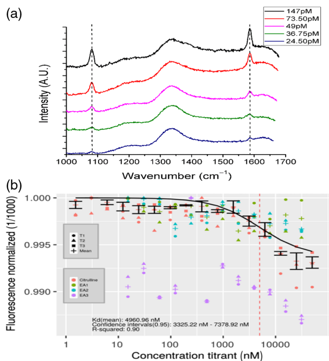
Fig. 4 (a) Serial dilution of functionalized nanocubes. (b) MST binding curve for citrulline aptamers. T1, T2, and T3 represent each test run on the MST. The 20 amino acids were separated into three different samples EA1, EA2, EA3 are tested to see how they bind to the citrulline aptamer.
