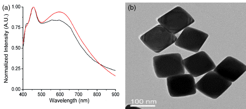
Fig. 2 (a) UV/VIS spectrum of Ag nanocubes (black line) and functionalized Ag nanocubes (red line). (b) TEM image of Ag nanocubes.
