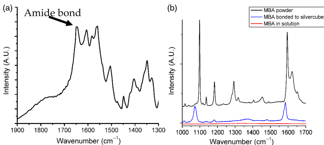
Fig. 3 (a) FTIR spectrum of functionalized Ag nanocubes, highlighting the amide bond formed between PEG and citrulline. (b) Raman spectrum of MBA powder (top plot) and SERS spectrum of 22.3 \mu\text{M} MBA bonded to Ag nanocubes (middle plot). Raman spectrum of 22.3 \mu\text{M} MBA dissolved in PBS showing no detectable signal at this concentration as expected (bottom plot).
