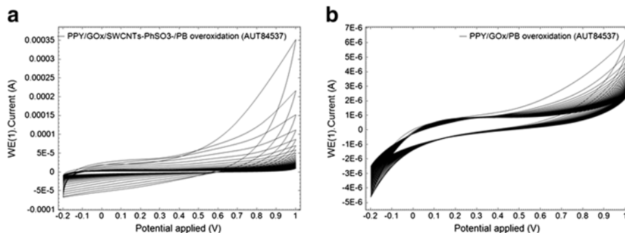
Figure 3 Cyclic voltammograms corresponding to overoxidation. PPY/GOx/SWCNTs- PhSO_3^- /PB (a) and PPY/GOx/PB (b) films in a 0.1 M phosphate buffer solution (pH 7.4), for a scan rate of 0.05 \text{ V s}^{-1} .
