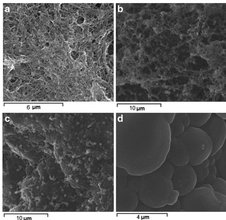
Figure 7 SEM images. Functionalized SWCNTs (a), PPY/GOx/SWCNTs-PhSO 3 - composite films obtained galvanostatically at 0.1 mA cm -2 (b) and 0.5 mA cm -2 (c), and pure polymeric PPY (d).
