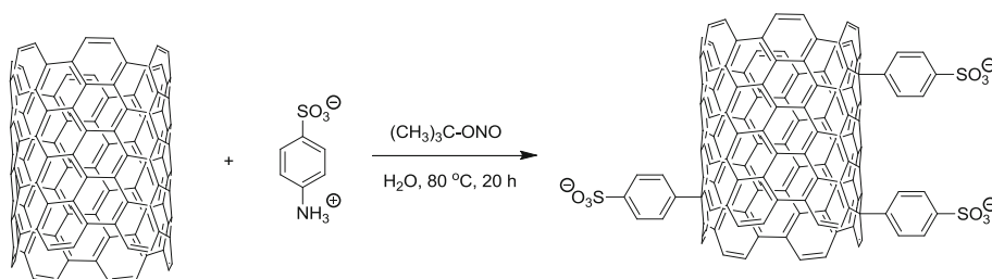
Figure 1 Functionalization of SWCNTs.
