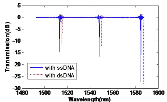
Fig. 3. (Color online) Simulation results of transmission spectra before (solid curve) and after (dashed curve) detection by double concentric ring resonators with a 5\text{ }\mu\text{m} outer ring radius when the probe is in the air gap.
