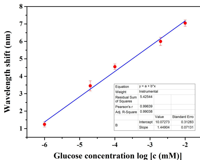
Fig. 10. Experimental results and deviation analysis of the spectral responses of the LPG biosensor integrated microfluidic chip to the change of glucose concentrations in three tests.
