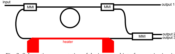
Fig. 3. Schematic representation of the integrated interferometric circuit
