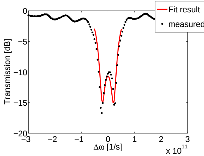
Fig. 2. Measured spectrum of all-pass microring with resonance splitting. The full line gives the theoretical transmission after fitting the model parameters
