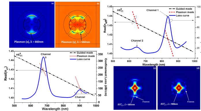
Fig. 2. Loss curve and dispersion relationship between the core guided mode and the plasmon modes at resonant wavelength. For x-polarized and y-polarized fundamental modes. (a) and (b) are magnetic field distributions of plasmon mode. (c) and (d) are magnetic field distributions of core guided mode at the resonance wavelength.
