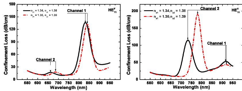
Fig. 4. Multi analyte operation of biosensor showing loss spectra of x and y polarizations of the fundamental modes ( HE_{11}^x and HE_{11}^y ). Attenuation peaks correspond to excited plasmons on the gold surface. The change of line type correspond to change in analytes in both runs.
