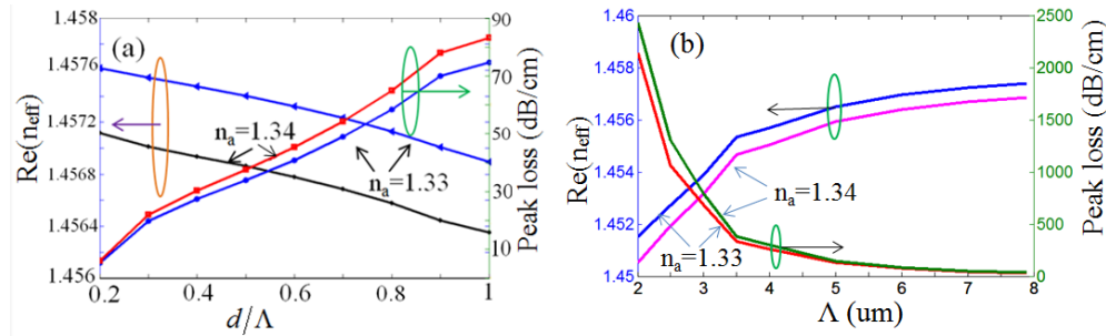
Fig. 4. The \text{Re}(n_{\text{eff}}) of the y-polarized core mode at the phase matching point and the peak loss of the y-polarized core mode for various values of (a) duty ratio with \Lambda = 7.9\text{ }\mu\text{m} , and h = 0.4\Lambda , (b) lattice pitch with d = h = 0.5\Lambda .
