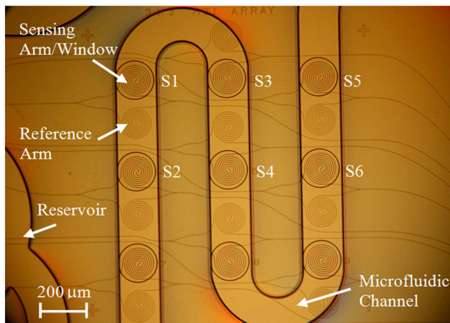
Fig. 1. (Color online) Top view of a silicon photonic wire MZI sensor array, with a monolithically integrated SU-8 microfluidic channel, that is aligned to the sensor windows for analyte delivery. The top six sensors (S1–S6) of the array are used in the experiment, while the bottom three sensors are independent test structures.
