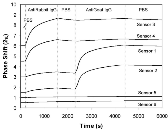
Fig. 2. Binding curves obtained using an IR camera to simultaneously track the phase change induced in the MZI sensors. Sensors 1 and 2 were printed with goat IgG, sensors 3 and 4 were printed with rabbit IgG, and sensors 5 and 6 were printed with BSA using a microarray spotter. For clarity the sensor response curves have been offset in the plot.
