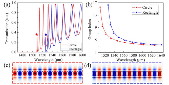
Fig. 2. (a) Simulated transmission spectra of slow light PhC waveguides with circular holes (red) and rectangular holes (blue). (b) Correspondingly derived group index contour of each PhC design. The propagation modes with the highest group index are marked by a star sign in (a), and their simulated mode profiles are shown in (c) and (d) for the circular hole and rectangular hole unit cell designs, respectively.
