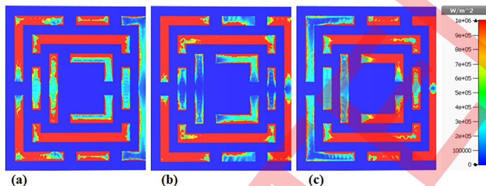
Fig 13. An examination of the surface power loss at: (a) at 0.684 THz, (b) at 0.918 THz, and (c) at 0.971 THz.
