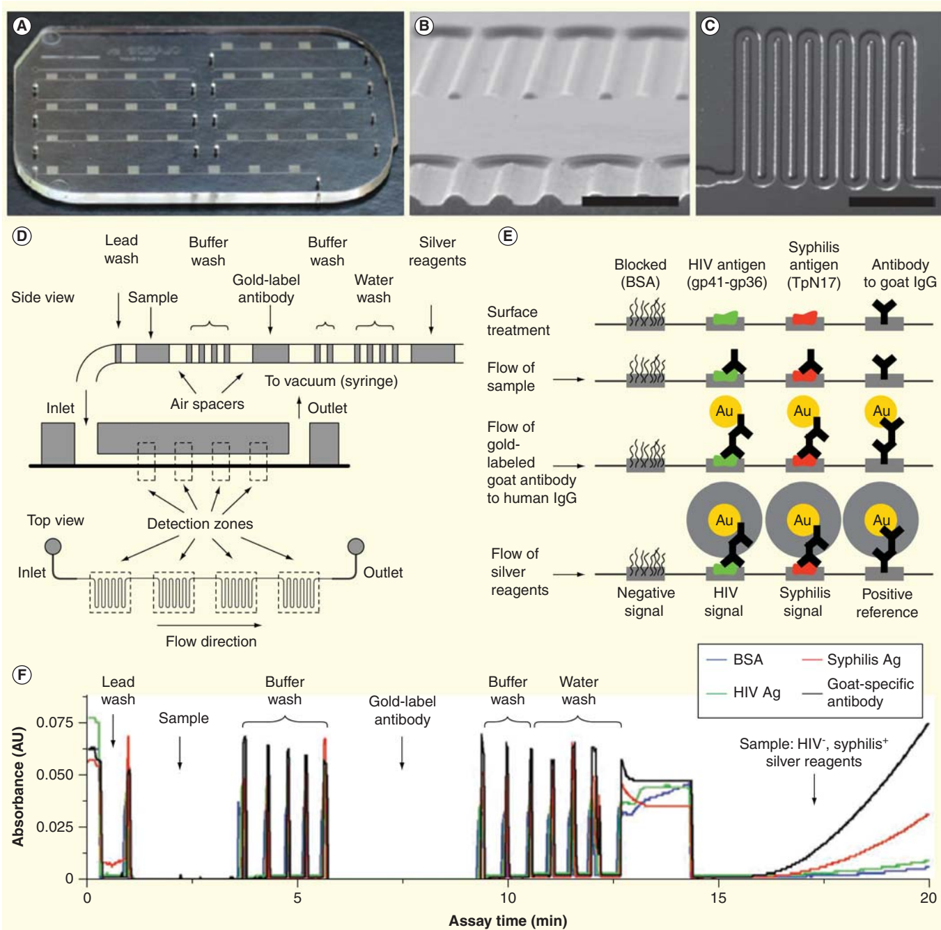
Figure 2. Integrated microfluidic system for multiplexed detection of HIV and syphilis. (A) Photograph of microfluidic chip. (B) Cross-section of microchannels. Scale bar, 500 μm. (C) The design of channel meanders. Scale bar, 1 mm. (D) Schematic diagram of passive fluid delivery of preloaded reagents over four detection zones based on vacuum generated by a disposable syringe. (E) Illustration of reactions at different detection steps. Signal amplification was achieved by the reduction of silver ions on gold nanoparticle-conjugated antibodies. Signals can be read quantitatively with low-cost optics or qualitatively by eyes. (F) Real-time monitoring of absorbance signals at the detection zones.
