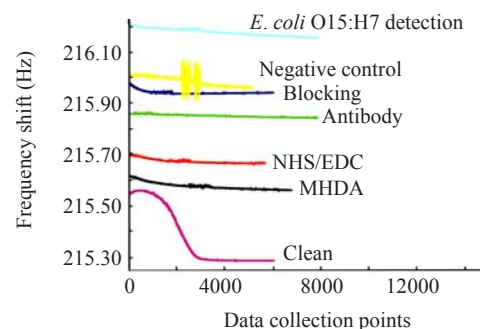
Fig.5 Temporal response curves of each step of the immunosensors fabrication and detection
