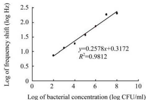
Fig.7 The logarithm graph for the frequency shift vs bacterial concentration
