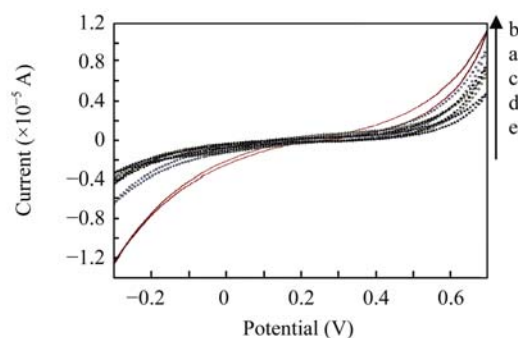
Fig.9 Cyclic voltammograms of the same Au electrode in the presence of 10 mmol/L [\text{Fe}(\text{CN})_6]^{3-/4-} for fabrication and detection. (a) MHDA-SAM; (b) EDC/NHS activation; (c) Antibody immobilization; (d) BSA blocking; (e) Bacteria binding
