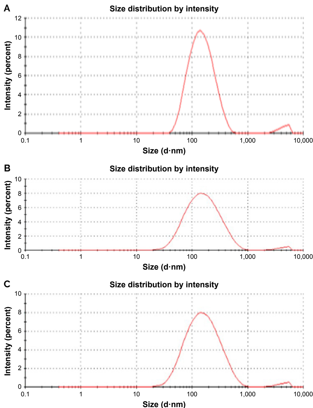
Figure 3 Particle size distribution of synthesized ZnO NPs using Albizia lebeck stem bark extract: (A) 0.1M, (B) 0.05M, and (C) 0.01M.
