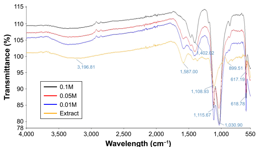
Figure 4 FTIR spectra of Albizia lebbbeck extract and synthesized ZnO NPs using various concentrations of zinc nitrate.
