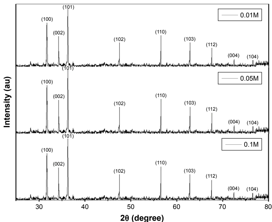
Figure 5 XRD pattern of 0.01M, 0.05M, and 0.1M synthesized ZnO NPs.
