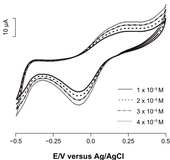
Figure 5 Cyclic voltammograms of biosensor immersed in epinephrine solutions of different concentrations ( 1 \times 10^{-5} \text{ M} , 2 \times 10^{-5} \text{ M} , 3 \times 10^{-5} \text{ M} , and 4 \times 10^{-5} \text{ M} ).
