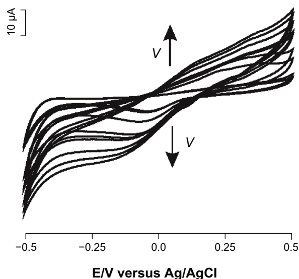
Figure 4 Cyclic voltammograms of biosensor immersed in 10^{-5} \text{ M} solution of epinephrine (supporting electrolyte phosphate-buffered saline, pH 7.0) registered at different scan rates, from 0.05 to 1.00 V per second.
