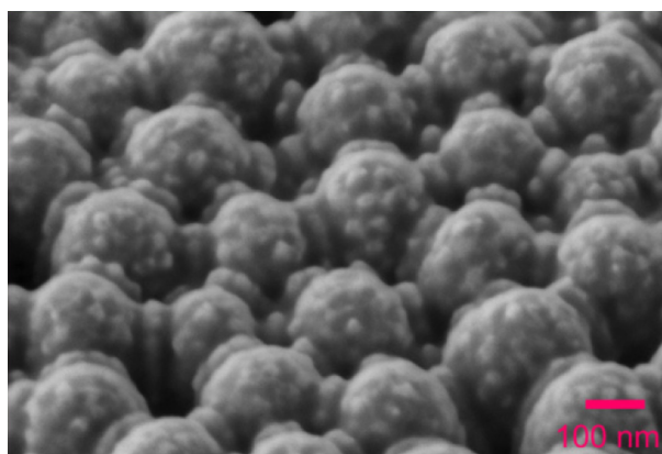
Figure 3 Scanning electron microscopic image of the GNP-deposited nanostructured electrode.
