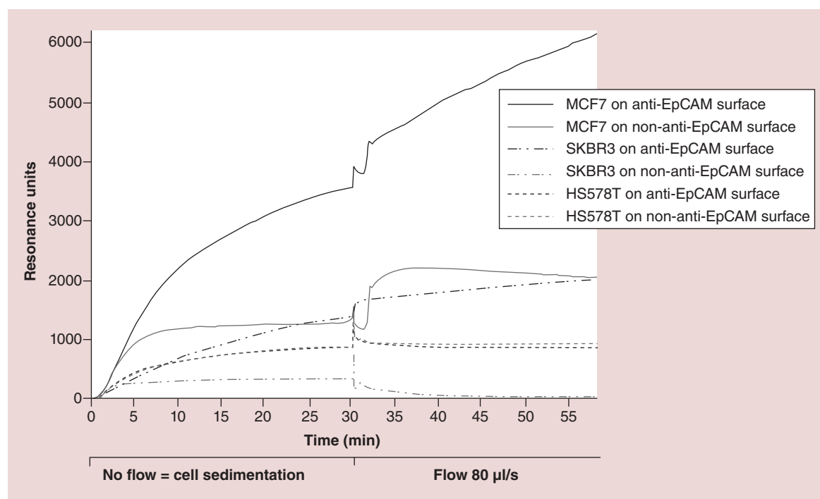
Figure 2. Surface plasmon resonance response of G-type biochip functionalized with 20 µg/ml epithelial cell adhesion molecule antibodies after the injection of MCF-7, SKBR3 and HS578T cells.
