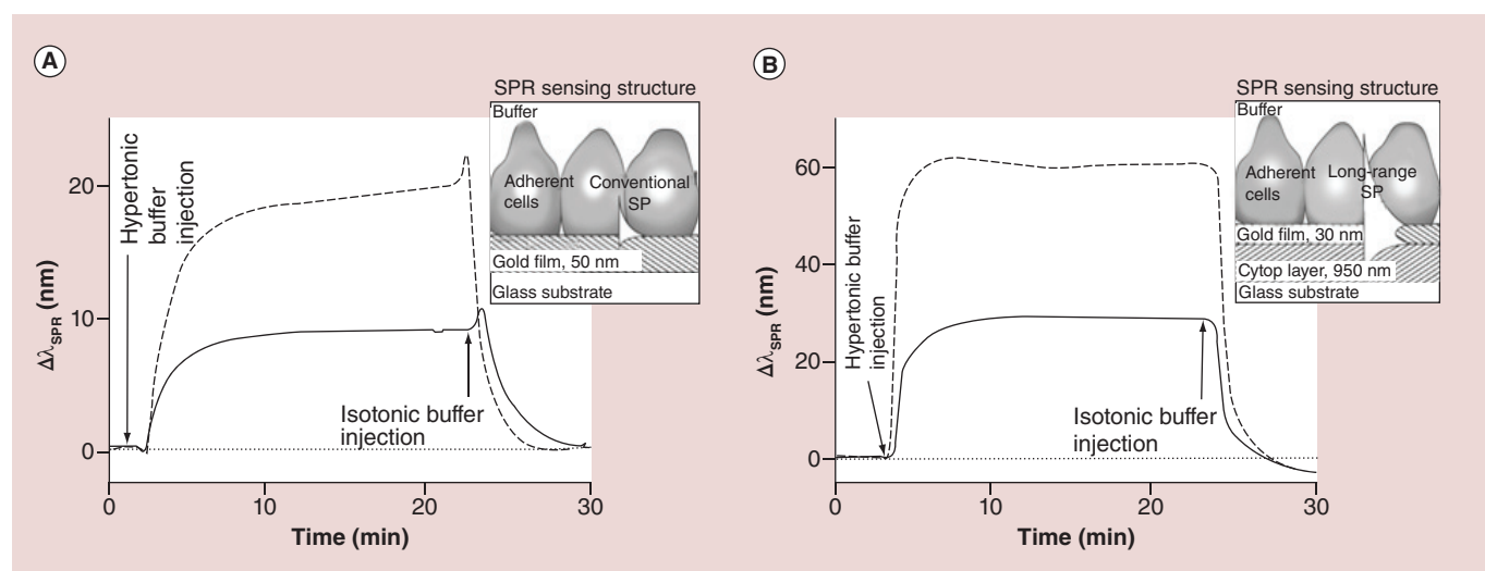
Figure 5. Conventional surface plasmon resonance and long-range surface plasmon resonance monitoring induced environmental changes to normal rat kidney cells. Surface plasmon resonance imaging kinetic response to a hypertonic solution exposed to confluent normal rat kidney cells by conventional SPR (A) and long-range SPR (B) that is provided by Dulbecco's phosphate-buffered saline ++ buffer supplemented with sucrose to give a 25-mM solution (solid line) or a 50-mM (dashed line) solution. SP: Surface plasmon; SPR: Surface plasmon resonance. Reproduced with permission from [44].
