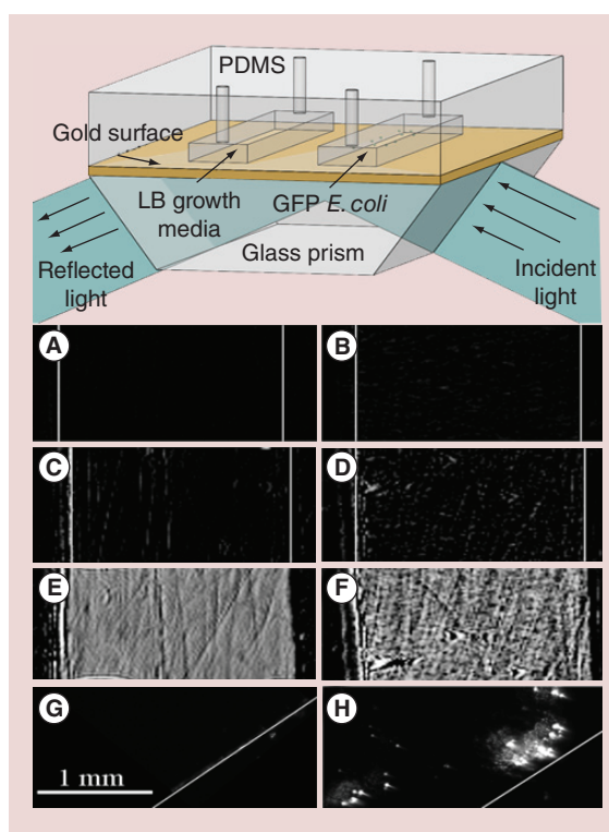
Figure 7. A study of biofilm formation using a custom microfluidic surface plasmon resonance imaging platform. (Top) A schematic representation of the surface plasmon resonance imaging experimental setup for measuring E. coli biofilm growth. (Bottom) Surface plasmon resonance imaging images of the blank chamber after (A) 6 min, (C) 1 h and (E) 6 h; GFP-labeled E. coli -filled chamber after (B) 6 min, (D) 1 h and (F) 6 h. Fluorescence images of the blank chamber (G) and of the GFP-labeled E. coli -filled chamber (H). LB: Lysogeny broth; PDMS: Polydimethylsiloxane. Reproduced with permission from [28].
