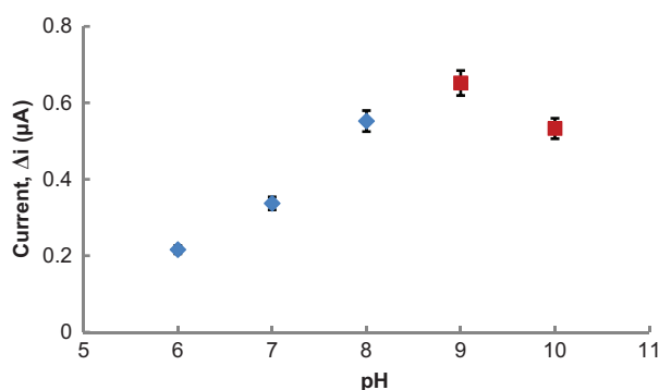
Figure 6. The effect of pH on the response of the biosensor (at 25°C, 1.0 \times 10^{-3} M Glu, at 0.3 V operating potential). (♦) 0.1 M phosphate buffer, (■) 0.1 M glycine buffer.
