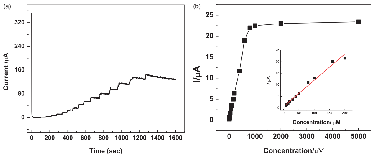
Figure 8. (a) Chronoamperometric responses of Lac- \alpha -Fe 2 O 3 NCs-CPE on successive addition of different concentrations and volumes of catechol solutions into pH 7, 0.2 M of PBS solution at an applied potential of 0.3 V; (b) Calibration curve with nonlinear fitting for Lac- \alpha -Fe 2 O 3 NCs-CPE response. Inset: Calibration curve with linear fitting.
