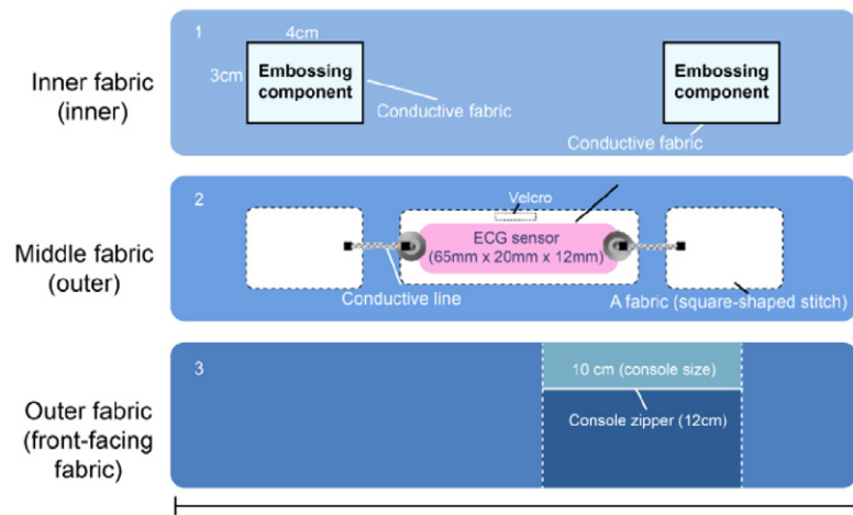
Fig. 2. Internal circuit design of the smartwear outdoor shirt on inner, outer, and front-facing fabric.
