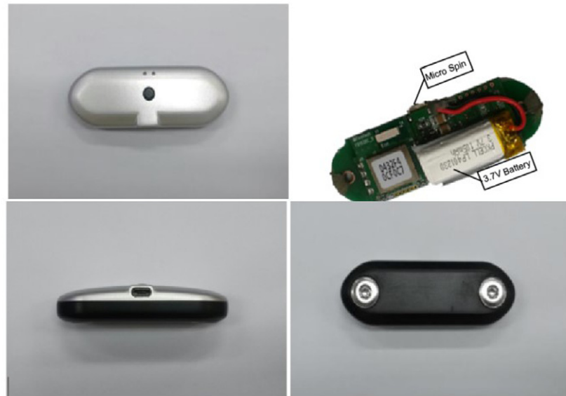
Fig. 3. Minimal-awareness ECG sensor for bioshirt.
