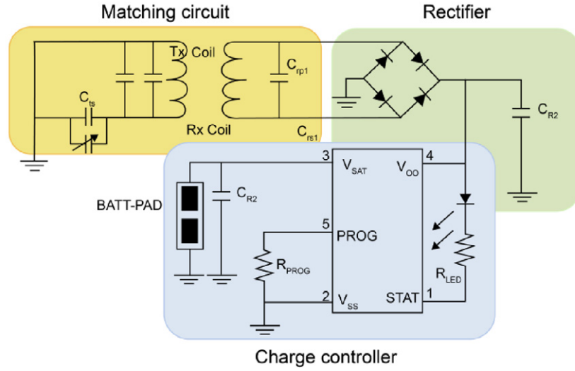
Fig. 4. Circuit diagram of wireless electric power transfer system.
