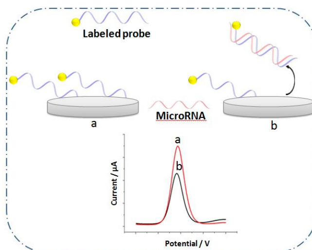
Figure 2. Architecture of electrochemical biosensor based on destroying the adsorption of the labeled probe after hybridization step on the electrode surface (a) before and (b) after hybridization.
