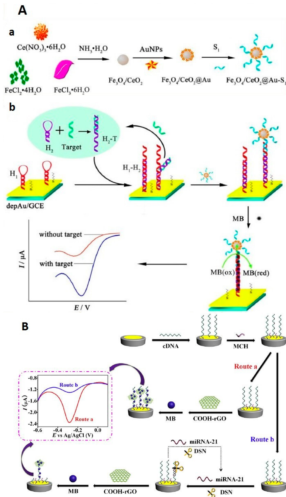
Figure 13. Example of biosensors using amplification strategy with nanomaterials as a non-nanocatalyst; (A) the nanomaterials are formed with \text{Fe}_3\text{O}_4 and cerium dioxide ( \text{CeO}_2 ) decorated with gold nanoparticles ( \text{Fe}_3\text{O}_4/\text{CeO}_2@\text{AuNPs} ) reproduced from [146] with permission of the publisher; (B) biosensors using graphene oxide and DSN as amplification method from [147] reproduced with permission of the publisher.
