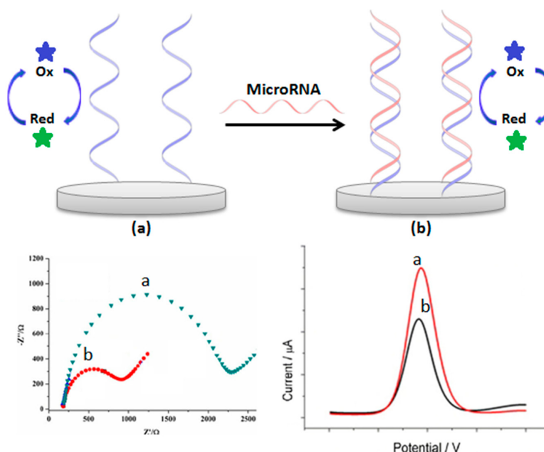
Figure 14. Electrochemical biosensors based on free RedOx indicator (a) before and (b) after hybridization.
