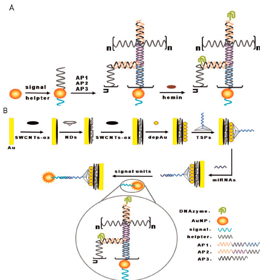
Figure 11. (A) DNA-functionalized AuNP based hybridization chain reaction, (B) Schematic illustration of miRNA biosensor using layered nanostructure of oxidized single-walled carbon nanotubes and nanodiamonds by hybridization chain reaction (reproduced with permission from the publisher) [129].
