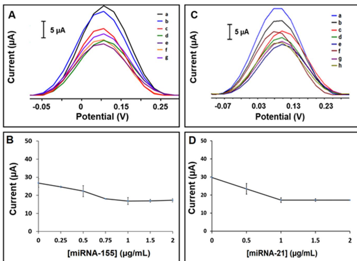
Figure 3. (A) Voltammograms representing the [\text{Fe}(\text{CN})_6]^{3-/4-} oxidation signal obtained by (a) Probe-1 immobilized AuNP/RGO-paper electrode in the absence of miRNA-155 target, after hybridization of Probe-1 with miRNA-155 target at concentrations of (b) 0.25 \mu\text{g/mL} , (c) 0.5 \mu\text{g/mL} , (d) 0.75 \mu\text{g/mL} , (e) 1.0 \mu\text{g/mL} , (f) 1.5 \mu\text{g/mL} , and (g) 2.0 \mu\text{g/mL} . (B) The line graph based on the average [\text{Fe}(\text{CN})_6]^{3-/4-} oxidation signal after hybridization between Probe-1 and miRNA-155 target with its various concentrations from 0 to 2.0 \mu\text{g/mL} ( n = 3 ). (C) Voltammograms representing the [\text{Fe}(\text{CN})_6]^{3-/4-} oxidation signals obtained by (a) Probe-2 immobilized AuNP/RGO-paper electrode in the absence of miRNA-21 target, after hybridization of Probe-2 with miRNA-21 target at concentrations of (b) 0.25 \mu\text{g/mL} , (c) 0.5 \mu\text{g/mL} , (d) 0.75 \mu\text{g/mL} , (e) 1.0 \mu\text{g/mL} , (f) 1.5 \mu\text{g/mL} , and (g) 2.0 \mu\text{g/mL} . (D) The line graph based on the average [\text{Fe}(\text{CN})_6]^{3-/4-} oxidation signal measured after hybridization between Probe-2 and miRNA-21 target with its various concentrations from 0 to 2.0 \mu\text{g/mL} ( n = 3 ).
