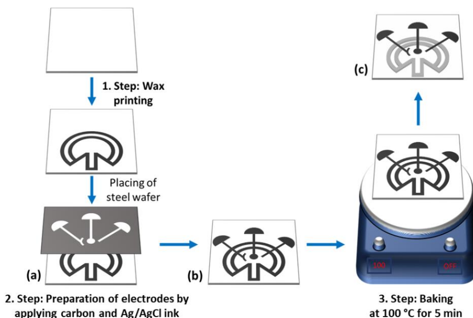
Scheme 1. Preparation of a paper electrode.
