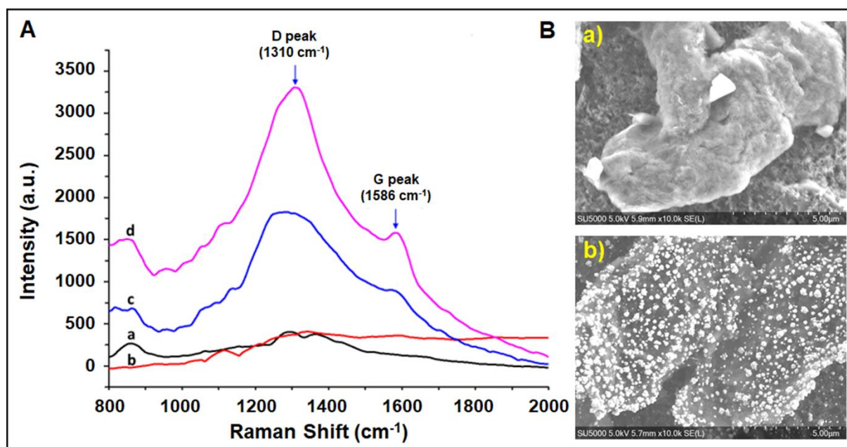
Figure 1. (A) Raman spectra of (a) nitrocellulose membrane (black), (b) carbon paste (red), (c) RGO-modified paper electrode (blue), (d) RGO-modified paper electrode after AuNP deposition (pink); (B) SEM images of (a) RGO and (b) AuNP/RGO-modified paper electrodes (scale: 5 μm). Gold deposition was performed with the chronoamperometric technique in aqueous solution of the HAuCl 4 gold precursor by applying −0.3 V for 10 min.
