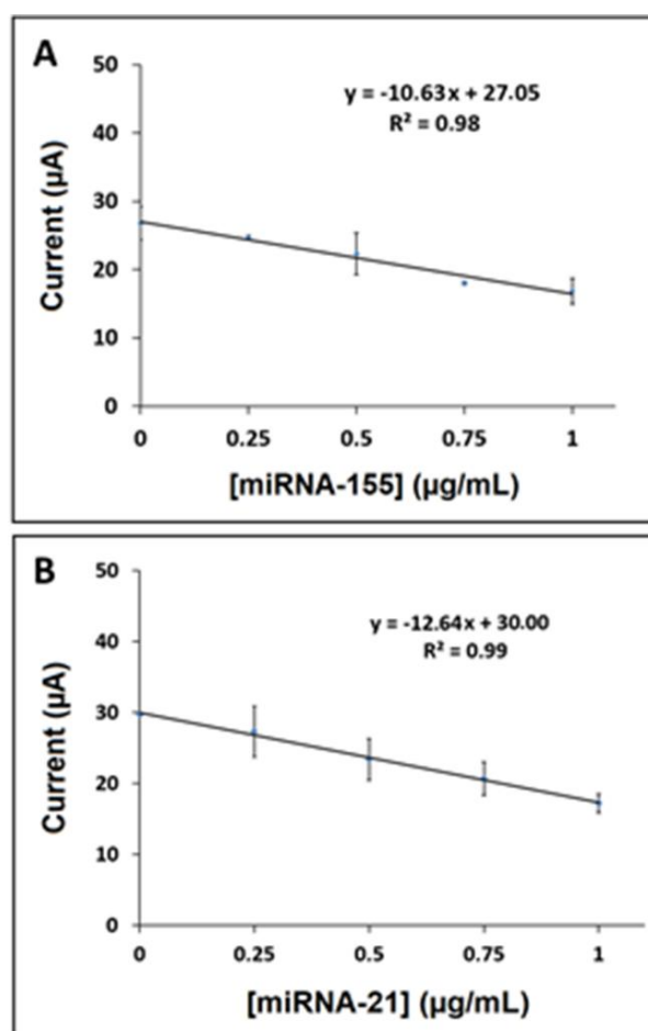
Figure 4. (A) Calibration plot for AuNP/RGO-paper electrode obtained after hybridization between Probe-1 and miRNA-155 target with its various concentrations from 0 to 1.0 µg/mL ( n = 3 ). (B) Calibration plot for the same electrode obtained after hybridization between Probe-2 and miRNA-21 target with its various concentrations from 0 to 1.0 µg/mL ( n = 3 ).
