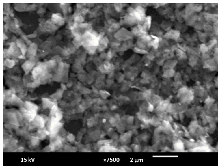
Figure 6. SEM image of MoS 2 nanosheets (scale: 2 μm).
